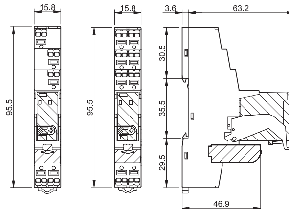
Types 4C.P1 / 4C.P2 Push-in terminals
