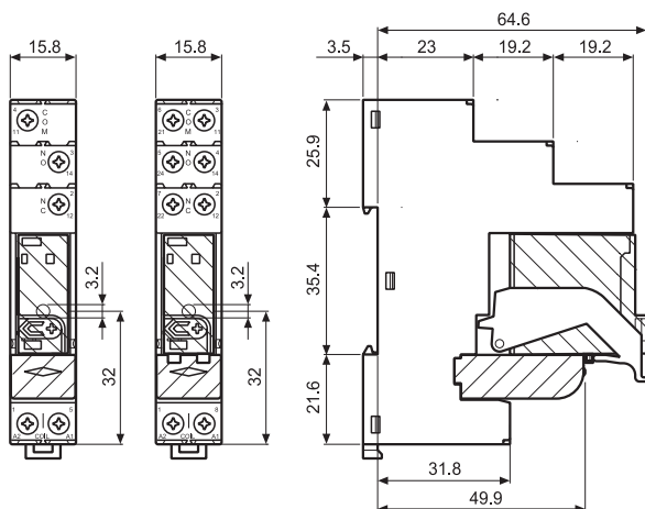
Types 4C.01 / 4C.02 Screw terminals
